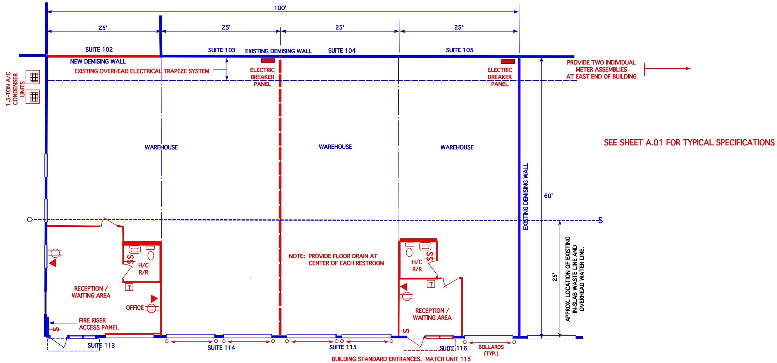
FLOOR PLAN
